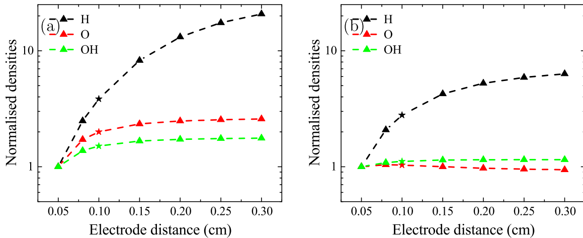
Figure 3. H, O, and OH densities, normalised to their values at d = 0.05 cm, as a function of inter-electrode distance for (a) 10 ppm and (b) 5000 ppm \text{H}_2\text{O} . The flow velocity is constant at 916 (a) and 966 \text{cm s}^{-1} (b). The power per unit volume is kept constant at 16.7 \text{ W cm}^{-3} for all points.
