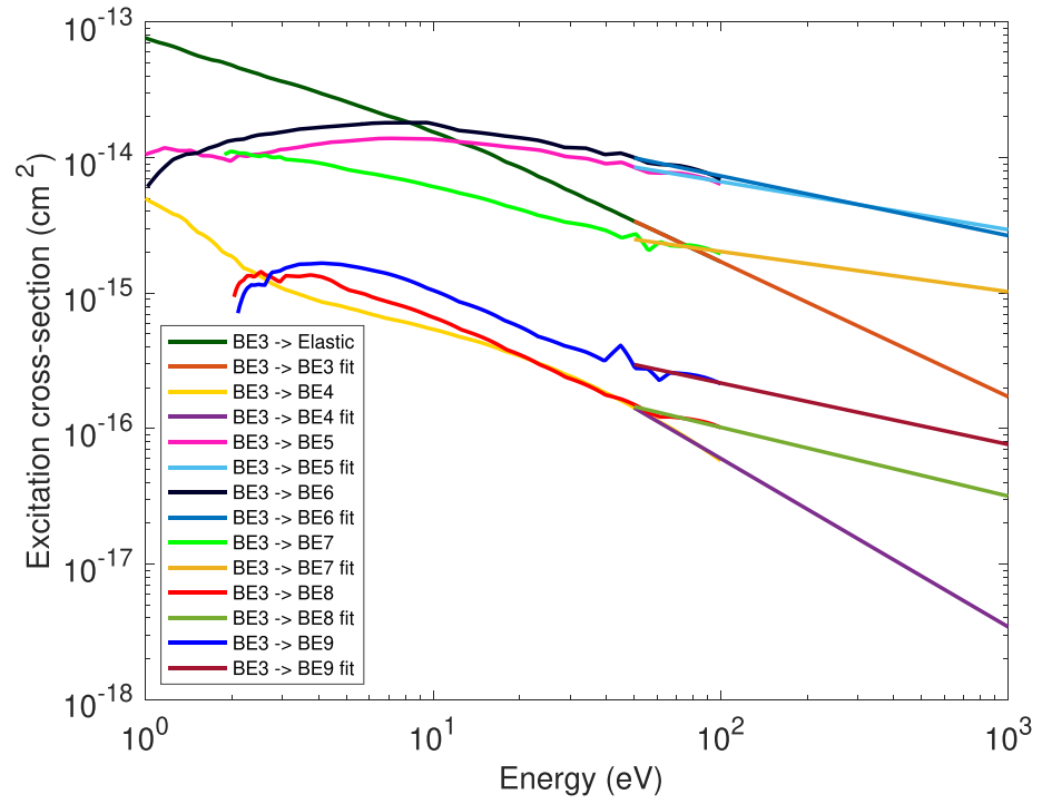
Figure A4. BE3 lumped state excitation cross-sections.
