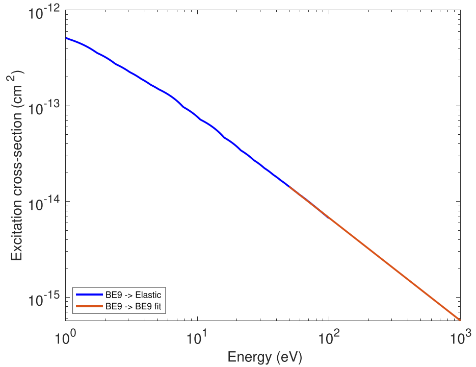
Figure A10. BE9 lumped state excitation cross-sections.
