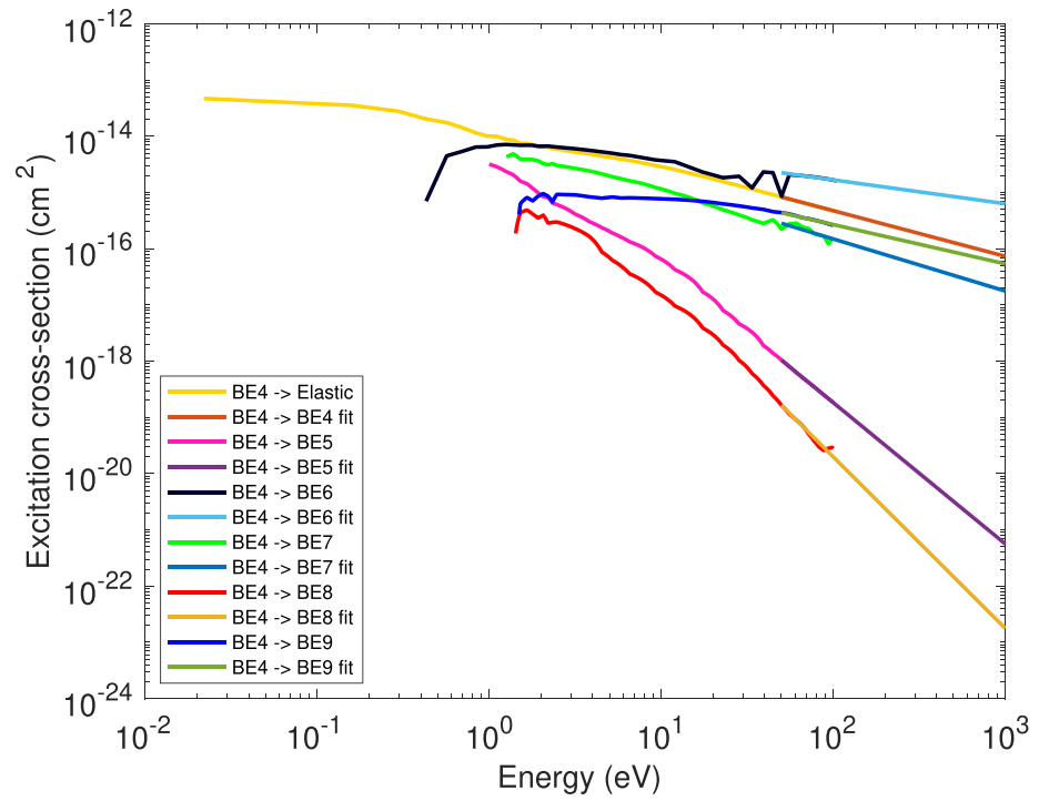
Figure A5. BE4 lumped state excitation cross-sections.
