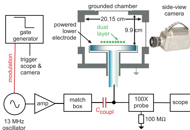
FIG. 1. Experimental setup. During plasma operation, the modulation signal was on, allowing rf power to be applied to the lower electrode, and a plasma was formed. Because of capacitor C_{\text{coup1}} , the lower electrode developed a negative dc self-bias. This self-bias helped electrically levitate grains in a 2D layer during plasma operation. When the modulation signal was switched off, the rf power extinguished, and at that moment an oscilloscope was triggered, and a side-view video camera began recording. Grains were illuminated by a vertical sheet of laser light, not shown here. During the afterglow, the lower electrode retained most of its negative dc bias due to the capacitor C_{\text{coup1}} . The bias on the lower electrode was measured using a Tektronix 100X probe. Its 100 \text{ M}\Omega impedance, in combination with C_{\text{coup1}} , provided a long discharge time constant of 3 s, so that a negative electrode bias remained throughout the afterglow.
