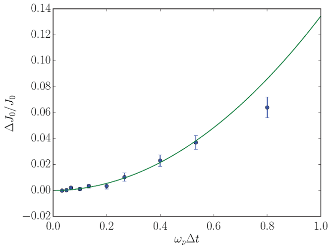
Figure 5. Verification by convergence toward an exact solution as a numerical parameter is changed. In this example, the physical parameter is the conduction current density flowing in a thermionic diode, and the numerical parameter is the time step in a particle-in-cell simulation. The points with error bars are simulation data, and the curve indicates the expected rate of convergence, which is O(\Delta t^2) in this case. Reproduced from [94]. © IOP Publishing Ltd. All rights reserved.
