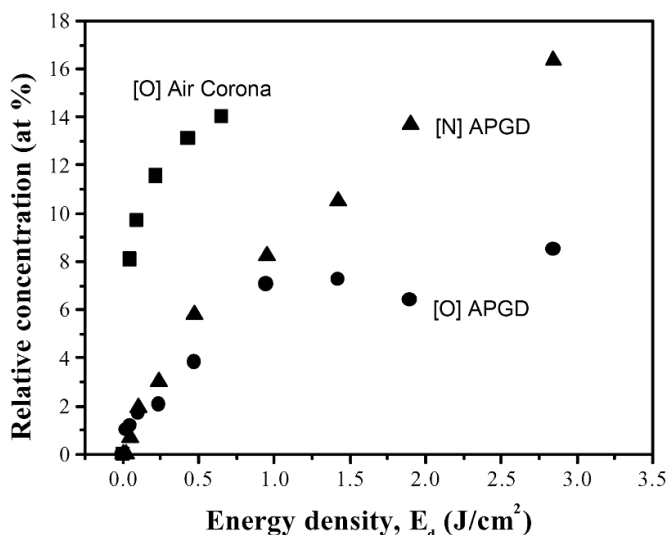
Figure 11. Surface concentrations of oxygen [O] and nitrogen [N] as a function of \text{J cm}^{-2} of plasma energy incident onto the surface after treating biaxially-oriented polypropylene (BOPP) using an air corona and an atmospheric pressure glow discharge (APGD) sustained in nitrogen. The repetition rate was 1 kHz. Reproduced from [202], with permission from Springer Nature.
