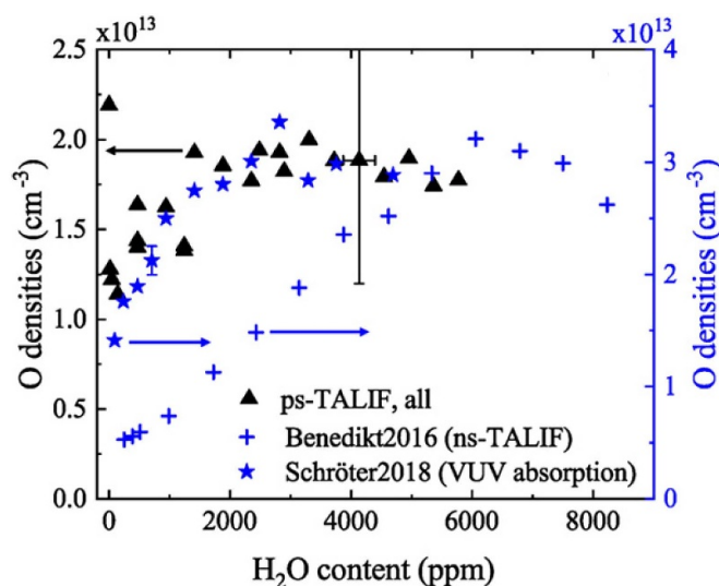
Figure 3. Comparison of measured absolute atomic oxygen densities in similar plasma sources using different diagnostic techniques: ns-TALIF [36], synchrotron VUV absorption [10] and ps-TALIF [37]. The plasma sources operate in a helium carrier gas flow through a 1 mm discharge gap with varying humidity admixtures. The power delivery is a RF-CCP at 13.56 MHz. Reproduced from [37]. © The Author(s). Published by IOP Publishing Ltd. CC BY 4.0 .
