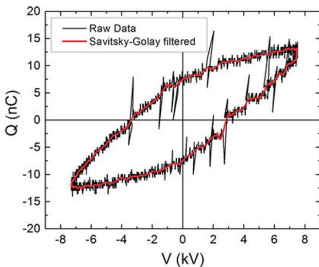
Figure 9. Example of filtered charge-voltage data, also known as a Lissajous plot, from a dielectric barrier discharge. Reproduced from [149]. CC BY 3.0.
